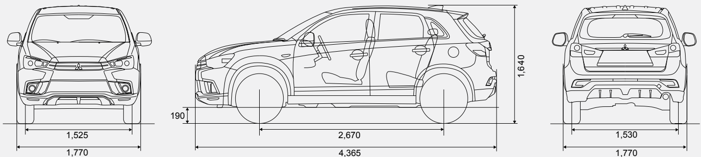
All measurements in millimetres
